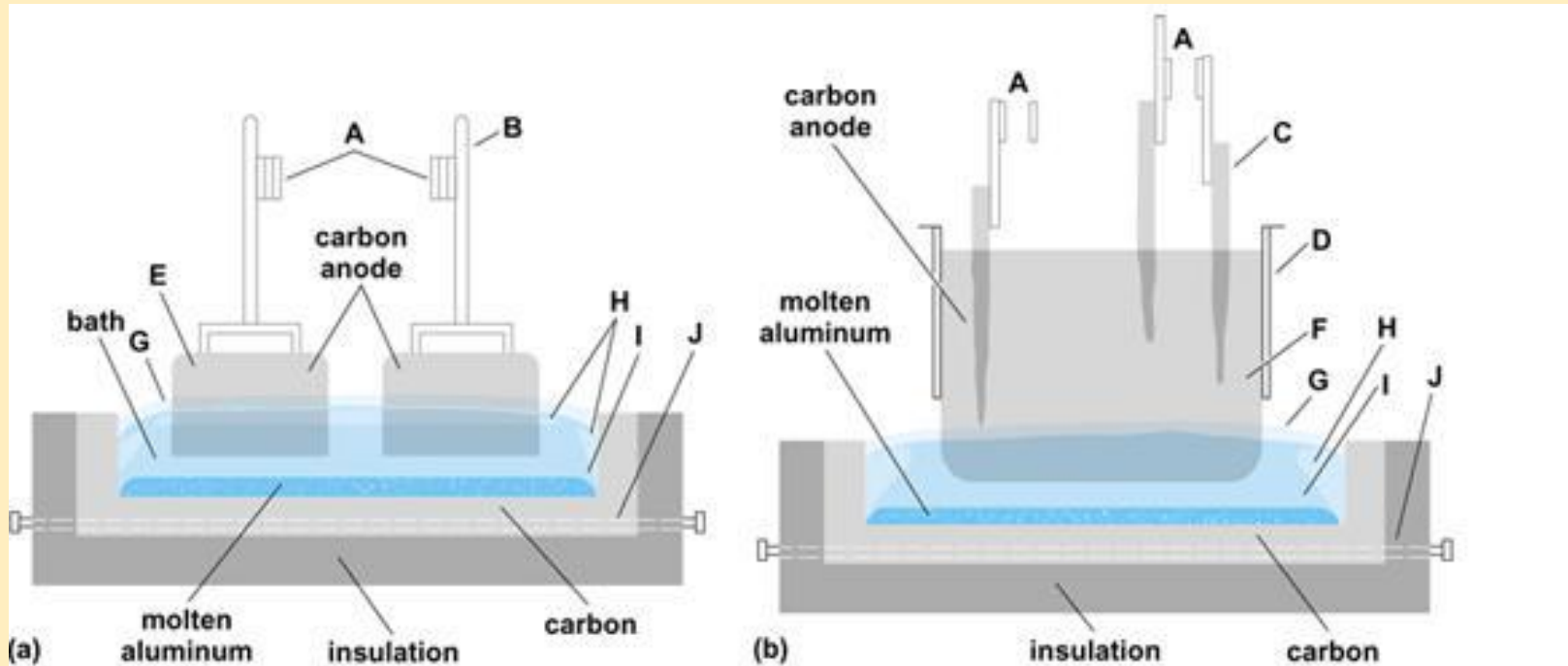
(a) Utilizing Prebaked Carbon Anode (b) Utilizing Soderberg(索德伯格) Carbon Anode
